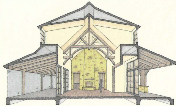
SECTION PERSPECTIVE
